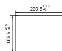
Panel cutout
