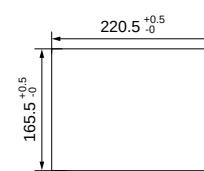
Panel cutout
