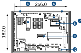
Rear view
